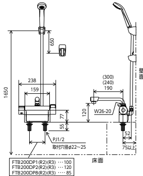
FTB200DP1 (2)(8)(R2)(R3) <取付工具 G4 >
